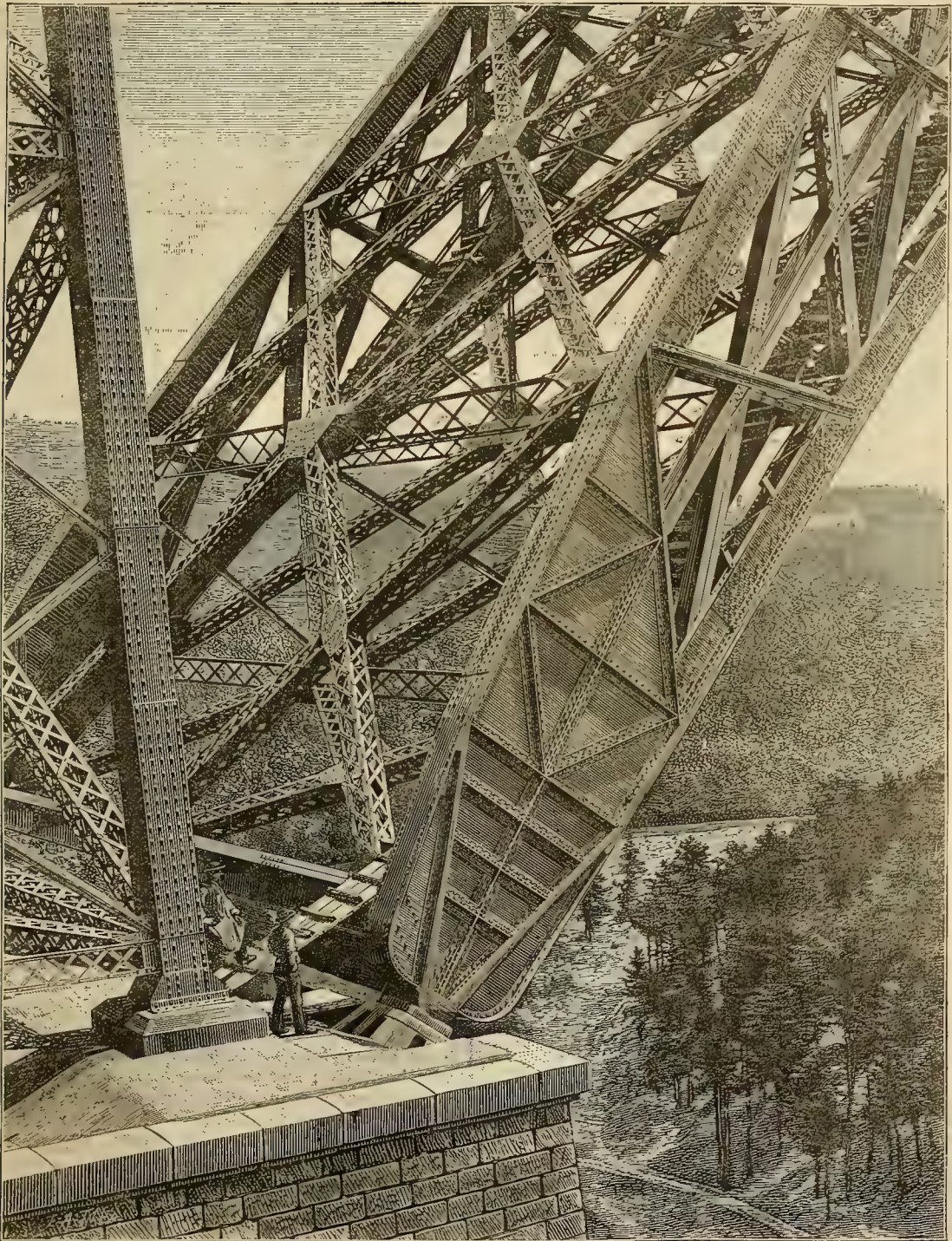
FIG. 3.—SPRING OF THE ARCH.
